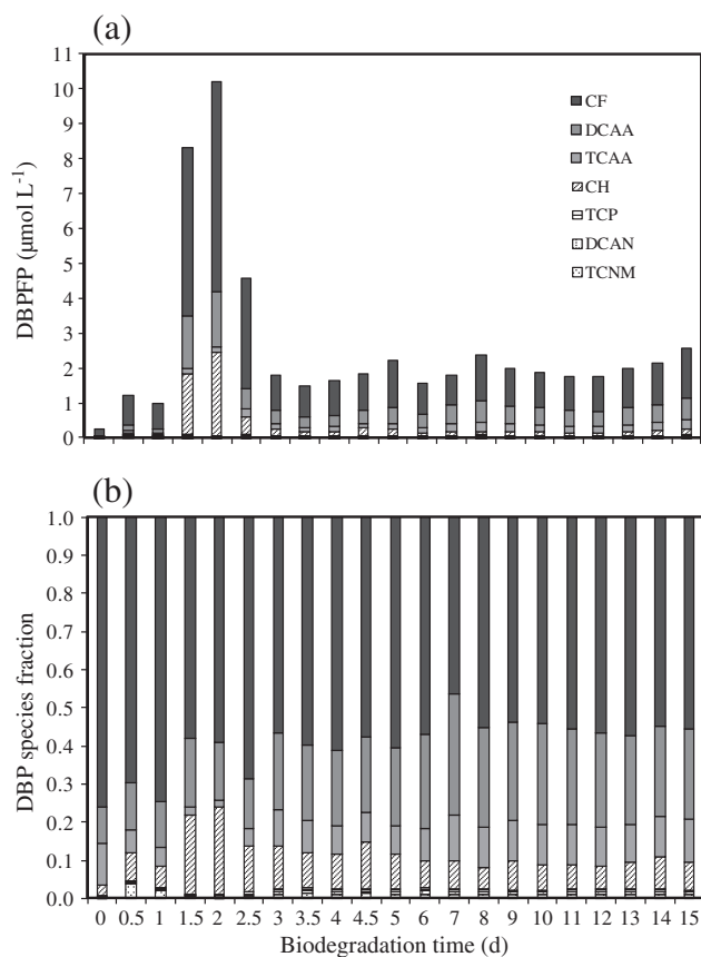
Fig. 2. (a) DBPFP and (b) DBP species fraction of the solution during organic biodegradation.
