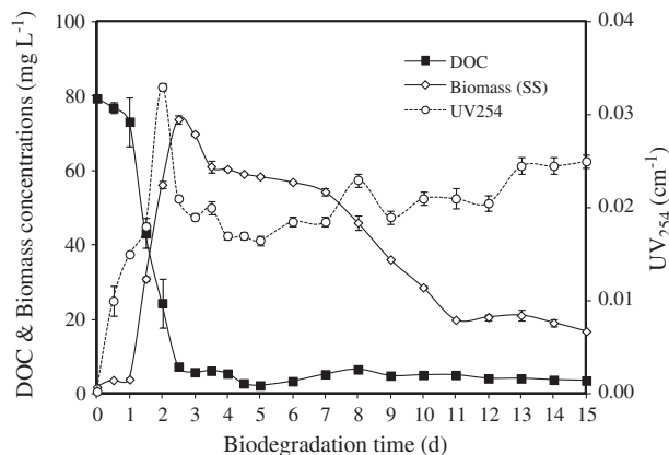
Fig. 1. DOC, biomass concentration, and UV 254 absorbance of the organic solution during the biodegradation test.
