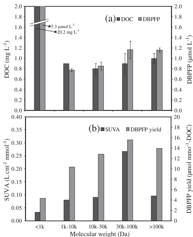
Fig. 5. (a) DOC and DBPFP and (b) SUVA and DBPFP yield of the SMP fractions of different molecular sizes from the day 5 sample.
