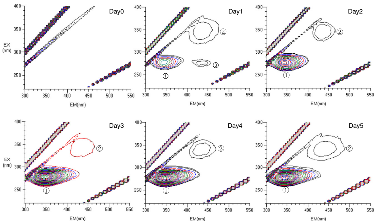
Fig. 4. FEEM of the organic matter in the SMP solution during organic biodegradation (① proteins, ② polycarboxylate-type humic acid, ③ polyaromatic-type humic acid).
