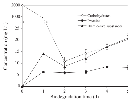
Fig. 3. Carbohydrate, protein, and humic-like substance contents of the organic matter in the SMP solution during organic biodegradation.
